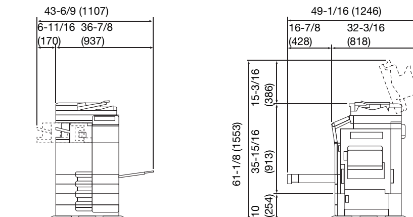
bizhub C368/C308/C258 + DF-704 + PC-210 + FS-533
