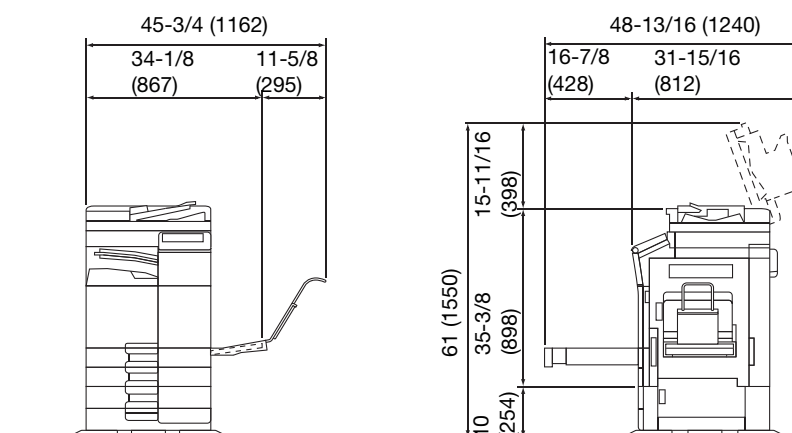
bizhub C368/C308/C258 + DF-629 + PC-210 + JS-506 + MK-730
